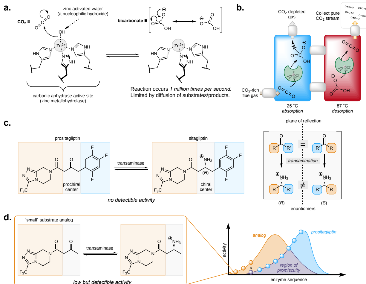
Fig 3. Re-optimizing enzymes to new conditions and substrate analogs. a. The reaction of carbonic anhydrase, a zinc metallohydrolase, which interconverts CO 2 and bicarbonate. b. Schematic of a carbonic anhydrase-catalyzed carbon capture system. c. Sitagliptin synthesis requires the installation of a chiral amine, which can theoretically be accomplished by a transaminase in a highly selective fashion, but no transaminase was identified to act on the precursor prositagliptin. d. A smaller prositagliptin analog was accepted by a transaminase (initial orange sphere), which could be evolved until an enzyme variant was identified with activity toward the full prositagliptin molecule (purple sphere). This could then be evolved into an industrially useful catalyst (blue spheres). This process is called a "substrate walk", and relies on substrate promiscuity—the ability of an enzyme to perform its reaction with a different substrate—and the selection of appropriate intermediate substrates.
